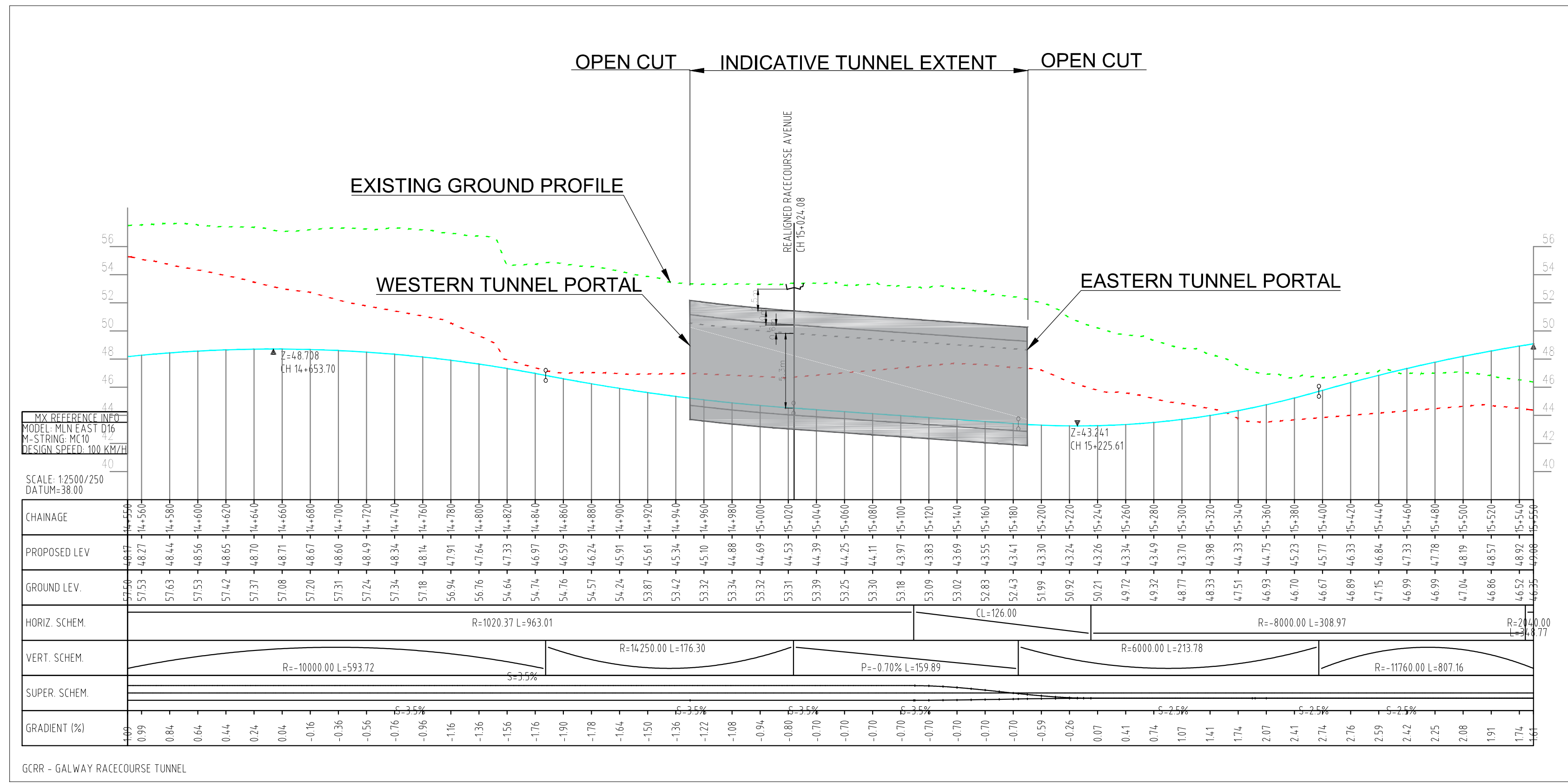
PROFILE VIEW
