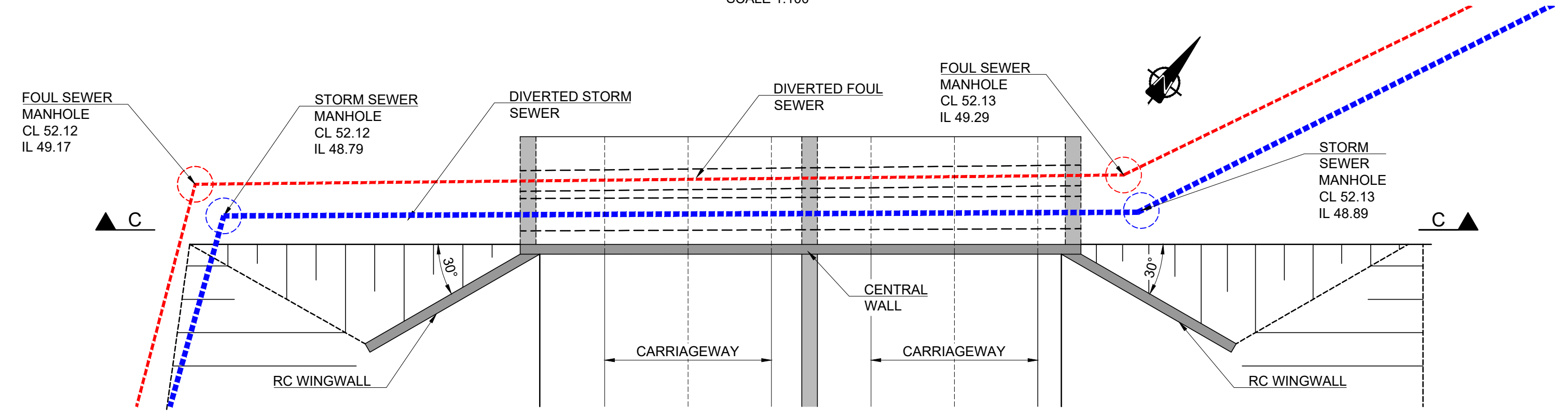
PLAN SE PORTAL- SERVICES DETAIL SCALE 1:200
