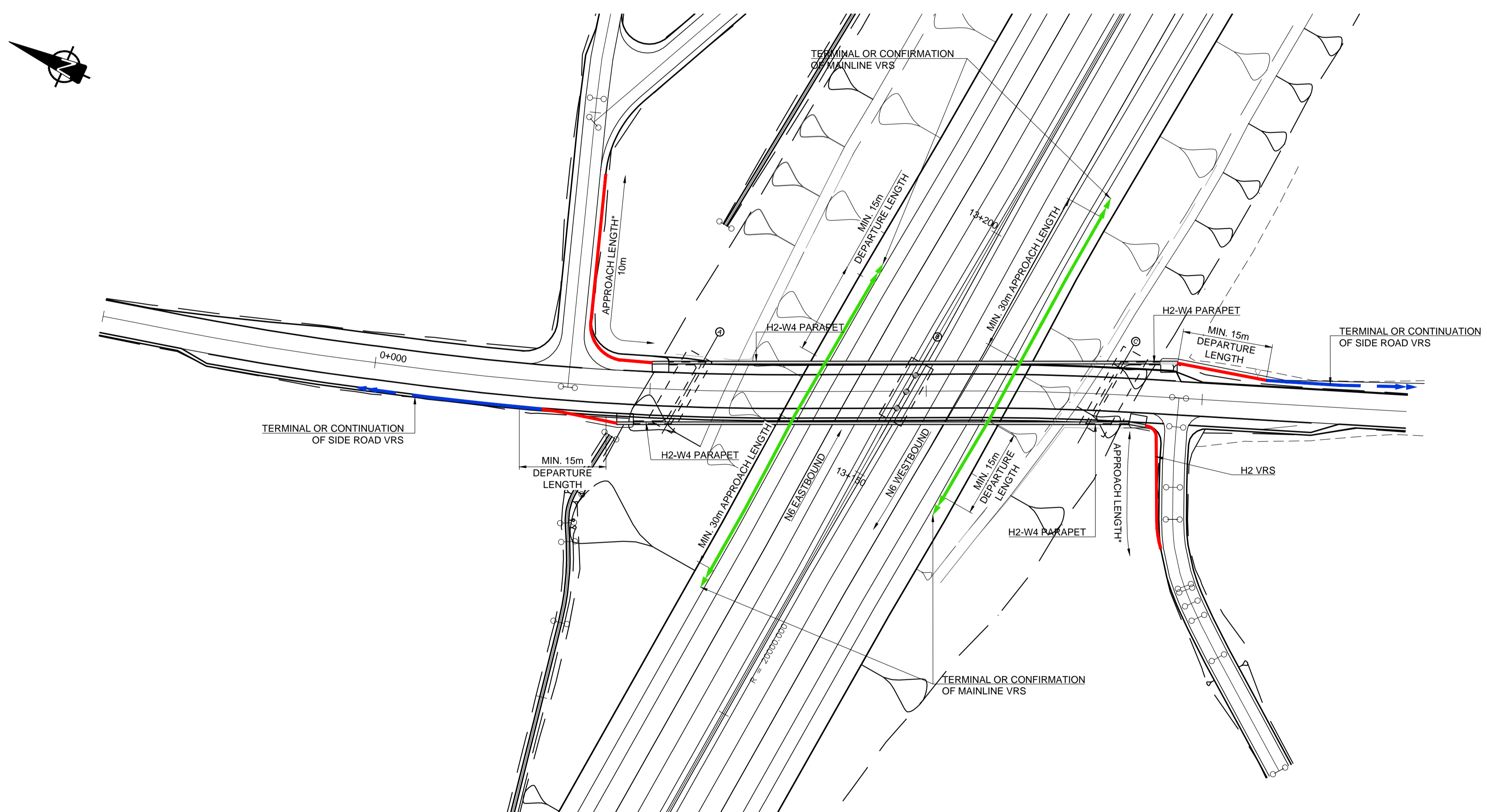
PARAPET / SAFETY BARRIER LAYOUT SCALE: 1:500
